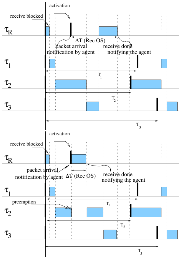
Figure 3. The model for the receive task in the TinyOS environment and with a FP scheduling.
