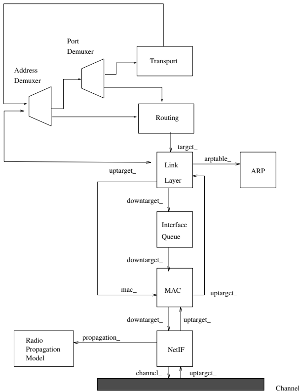
Figure 1. Architecture of a wireless node in NS-2.
