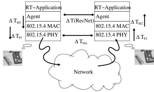
Figure 4. The agent-agent delay as computed using the ordinary NS-2 timing.
