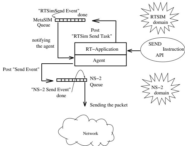
Figure 2. The send instruction API.
