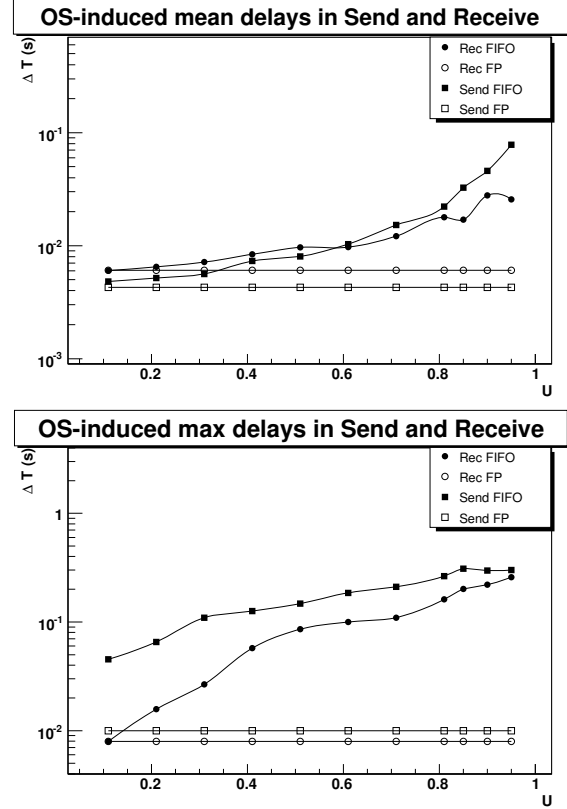
Figure 6. The mean and maximum delays in message elaboration due to the CPU activity as a function of the utilization factor for FCFS and FP scheduling policies.
