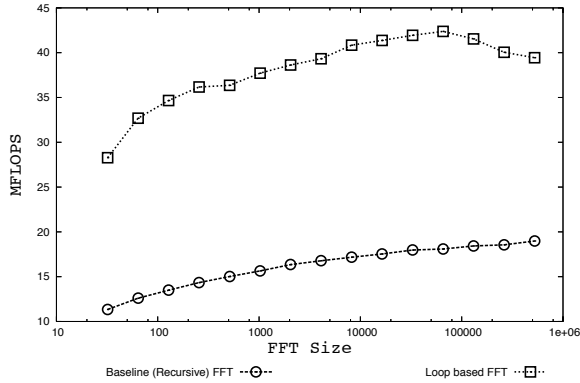
Figure 2: Comparison between a reentrant and a loop implementation of FFT
