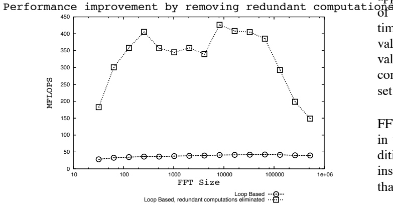
Figure 3: Improvement after removal of redundant computations
