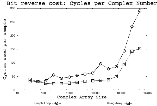
Figure 4: Comparison of the computational cost of bit reverse. Two implementations shown
