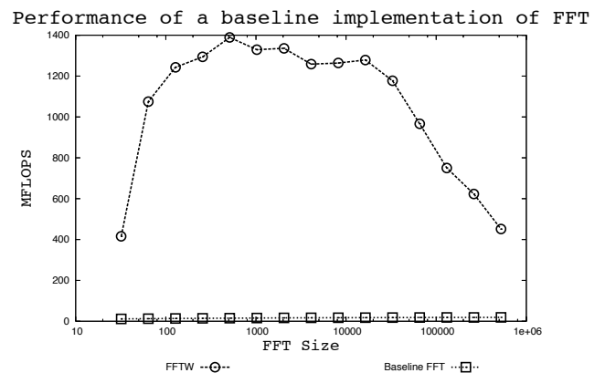
Figure 1: Comparison between a simple implementation of FFT and the commercial FFTW
