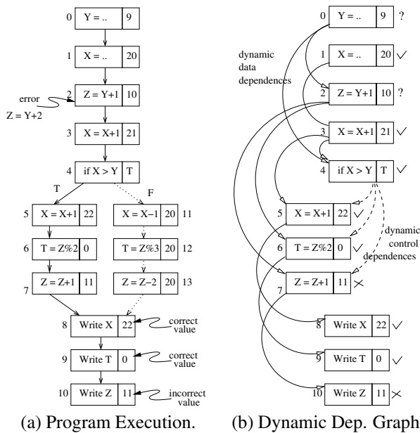
Figure 4. Pruning a dynamic slice.
