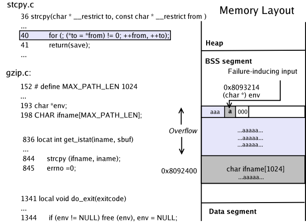
Figure 2. gzip Buffer Overflow.
