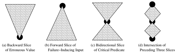
Figure 1. Types of Negative Evidence and Corresponding Dynamic Slices.
