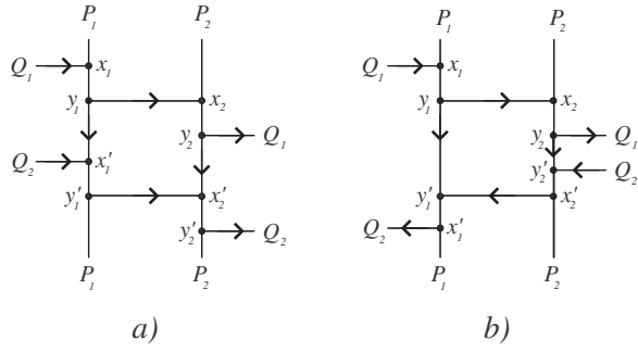
Figure 7. Crossing lemma impossibility
