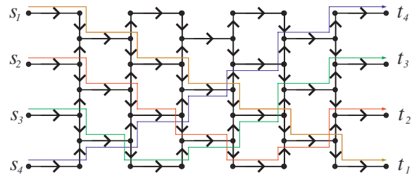
Figure 1. A pathological example
