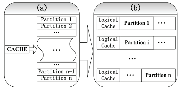
Figure 8. Cache organizations: (a) centralized cache; (b) distributed caches
