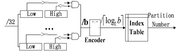
Figure 4. Schematics of the indexing logic.
