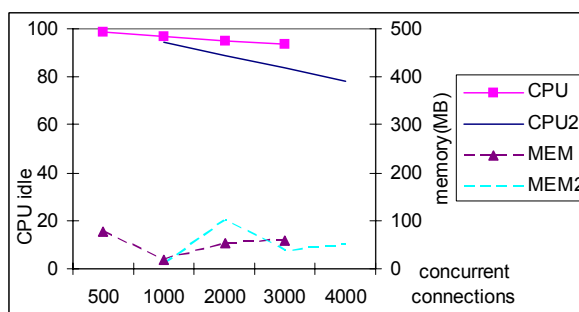
Fig. 6. Narada tests, CPU idle and memory consumption CPU and MEM are single server tests CPU2 and MEM2 are DBN tests
