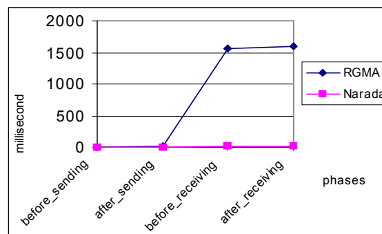
Fig. 15. RTT decomposition
