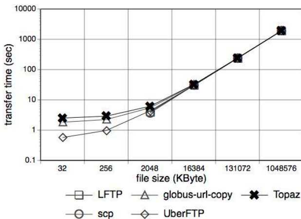
Figure 9. Transfer rate of upload (put)
