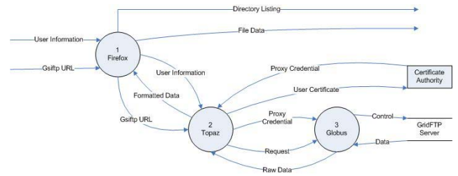
Figure 4. Level 1 DFD for download
