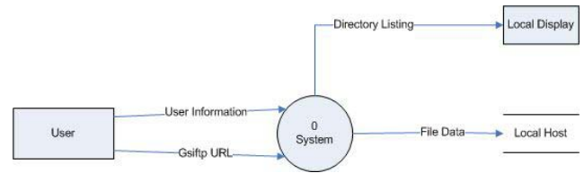
Figure 2. Level 0 DFD for download
