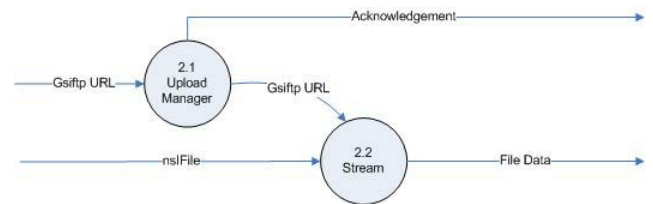
Figure 7. Level 2 DFD for upload
