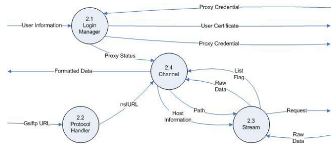
Figure 6. Level 2 DFD for download
