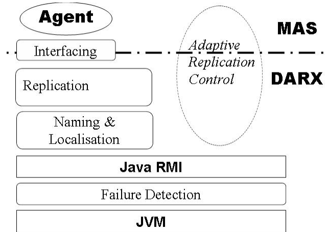
Figure 1. DARX framework design.
