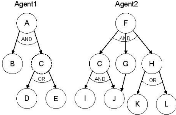
Figure 3. Example of plans of two interacting agents.
