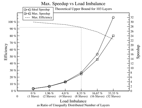
Figure 8. Impact of Load Imbalance
