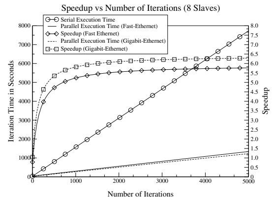
Figure 9. Speedup Depending on Iterations
