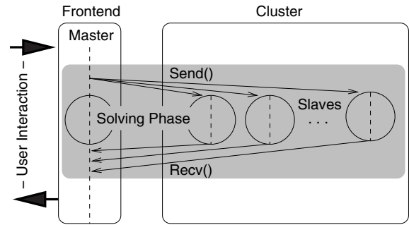
Figure 4. Master-Slave Concept
