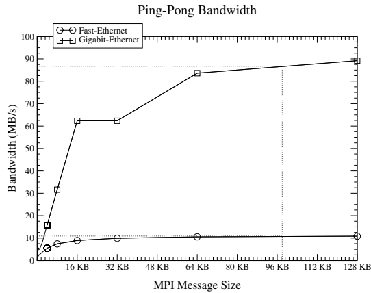
Figure 6. Ping-Pong Bandwidth
