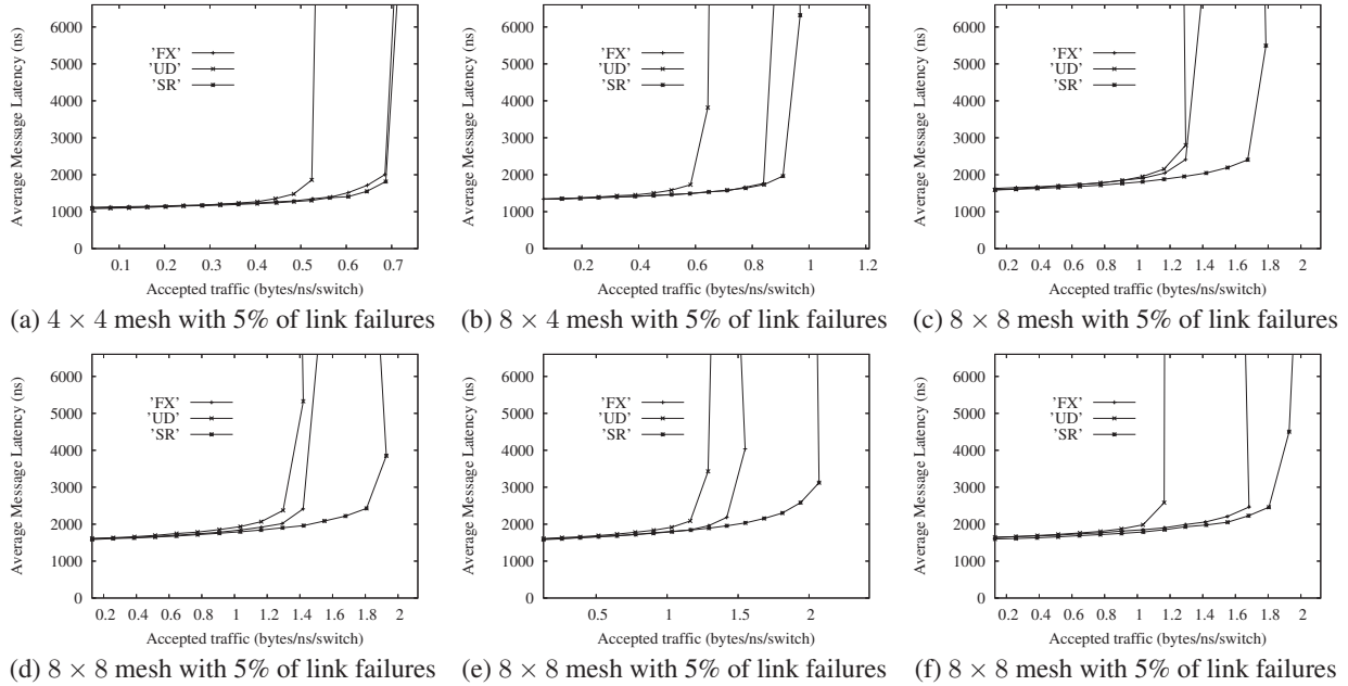
Figure 7. Average packet latency vs throughput. Uniform distribution of packet destinations.
