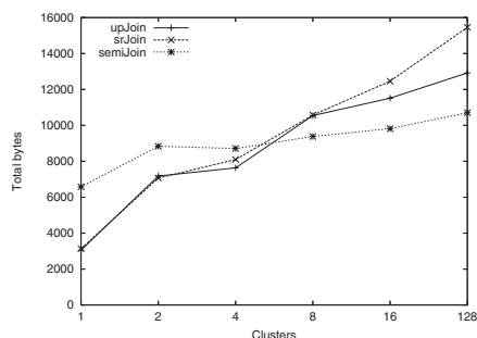
(b) UpJoin and SrJoin vs. SemiJoin
