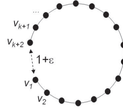
Figure 7. Example where UHI fails: nodes v_1 and v_{k+2} are separated by a path of k+1 hops, but are close (distance 1 + \epsilon ). Thus, concurrent transmissions of nodes v_2 and v_{k+2} may interfere at v_1 in spite of their large hop distance.
