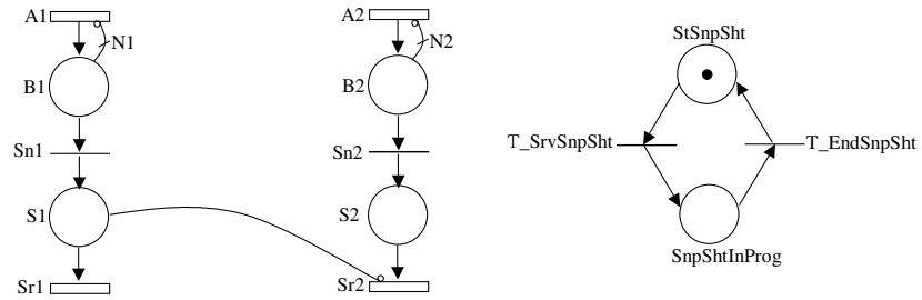
Figure 2. SRN model for the Reactor pattern
