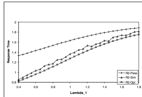
Figure 4. Response time as a function of \lambda_1
