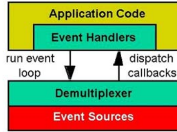
Figure 1. Event Demultiplexers in Middleware
