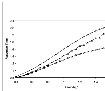
Figure 4. Response time as a function of \lambda_1
