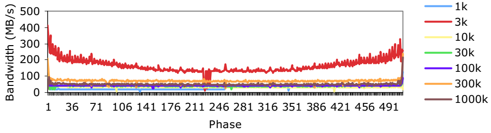
Fig. 7. Congested-controlled AAPC on 512-processor Columbia
