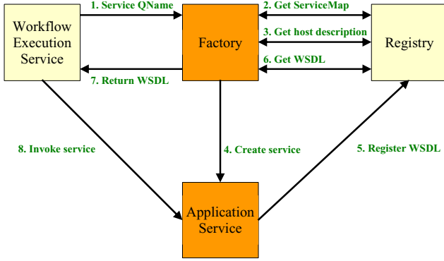
Figure 2. Just-in-time creation of application services using GFac
