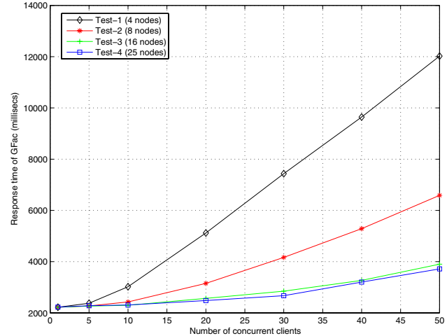
Figure 3. Response time of GFac
