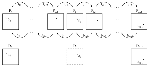
Fig. 1. Depth tracking from motion analysis
