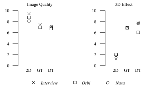
Fig. 4. Rating of image quality and 3D effect for the variants 2D , Ground Truth , Depth Tracking
