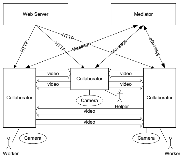
Figure 1. WebDOVE system architecture for one expert (helper) with two workers.
