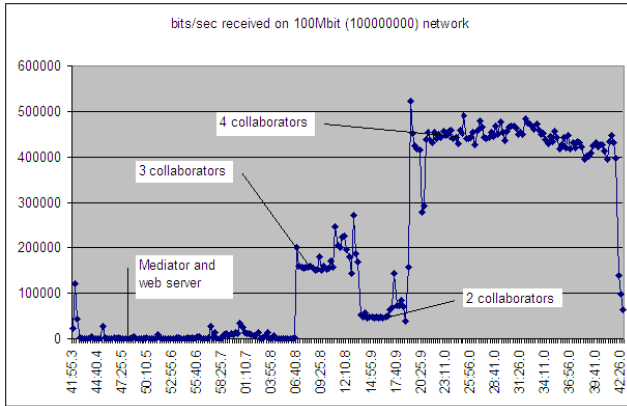
Figure 5. The network traffic of one participating computer. It runs the web server, Mediator, and a Collaborator.
