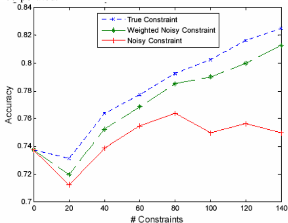
Figure 4. Accuracy with different numbers of constraint
