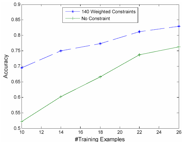
Figure 5. Accuracy with different sizes of training set
