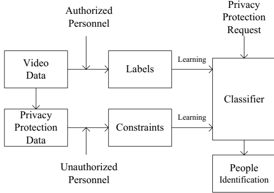
Figure 2. The flow chart of the learning process
