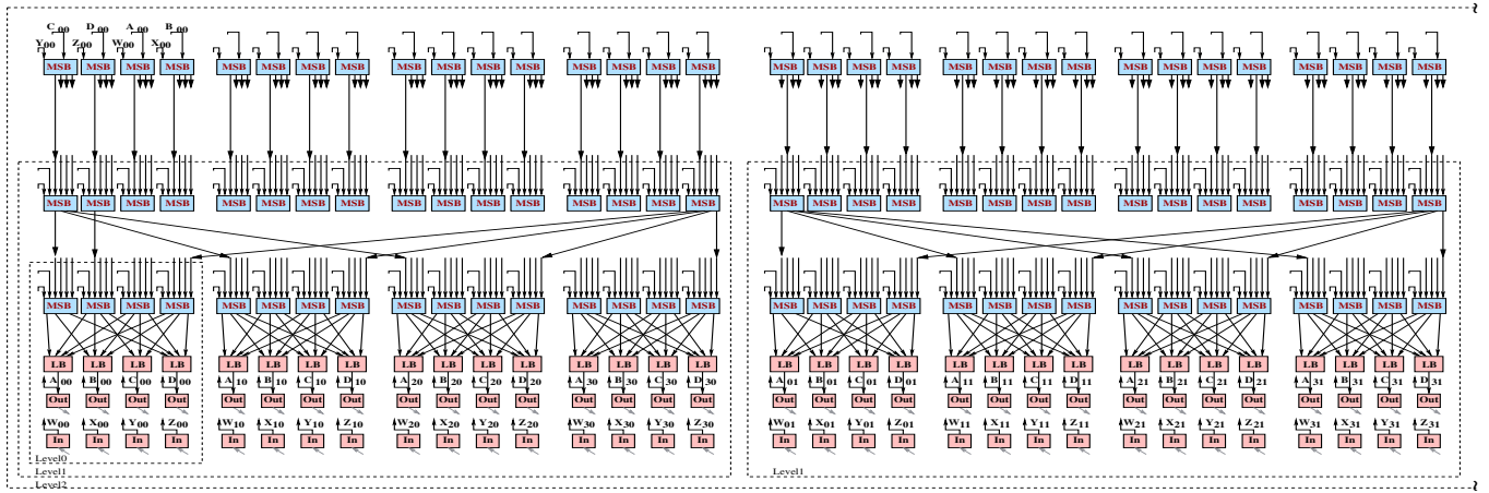
Figure 3: Three level MFPGA structure with k = 4 and p = 1
