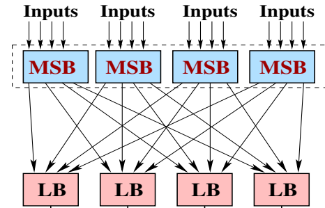
Figure 1: Downward Network in the Level 0 Cluster
