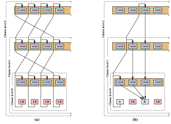
Figure 2: The Impact of the Upward Network
