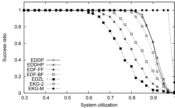
Figure 11: Success ratio: U_{max} = 1.0 , M = 4
