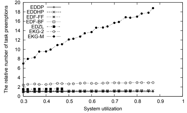
Figure 16: Task preemptions: U_{max} = 0.5 , M = 16
