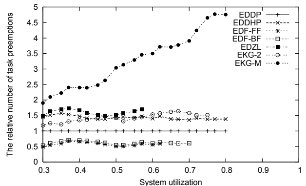
Figure 17: Task preemptions: U_{max} = 1.0 , M = 4
