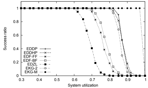
Figure 13: Success ratio: U_{max} = 1.0 , M = 16
