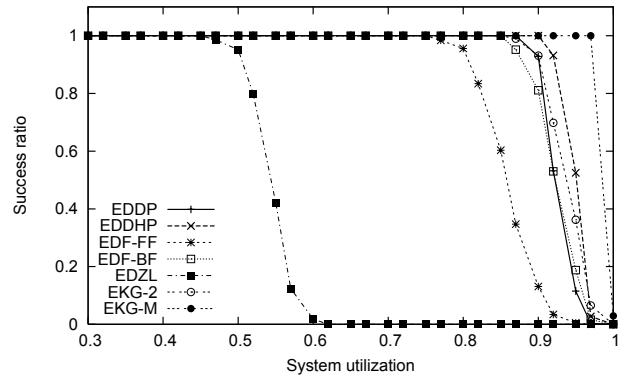
Figure 9: Success ratio: U_{max} = 0.5 , M = 8
