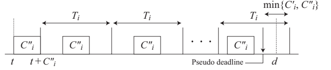
Figure 7: \tau_i'' consumes the most time
