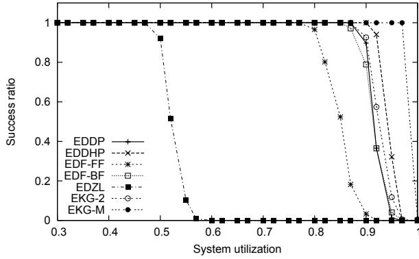
Figure 10: Success ratio: U_{max} = 0.5 , M = 16
