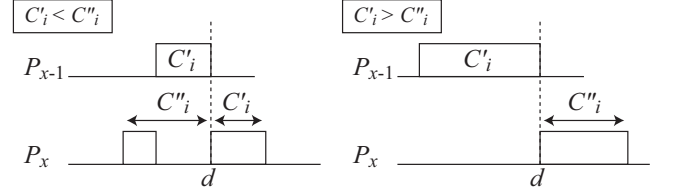
Figure 3: EDDP scheduling example
