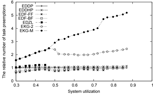
Figure 14: Task preemptions: U_{max} = 0.5 , M = 4
