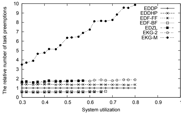
Figure 18: Task preemptions: U_{max} = 1.0 , M = 8
