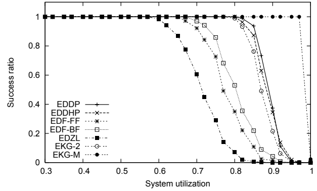
Figure 12: Success ratio: U_{max} = 1.0 , M = 8
