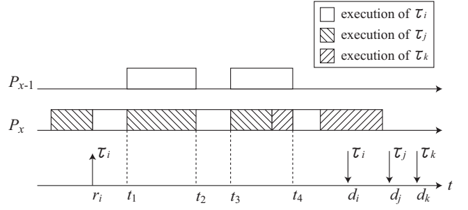
Figure 3: EDDP scheduling example
