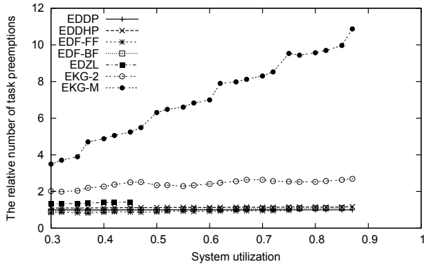
Figure 15: Task preemptions: U_{max} = 0.5 , M = 8
