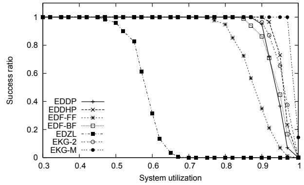
Figure 8: Success ratio: U_{max} = 0.5 , M = 4
