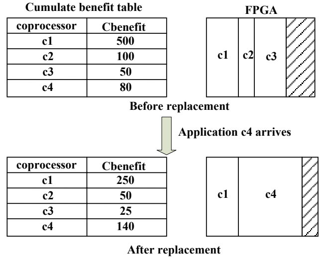
Figure 3: Coprocessor replacement policy in the fading cumulative benefit heuristic. The fading factor f is 0.5, tp4-tc4 is 100 cycles, loading time( c4 ) is 40 cycles.
