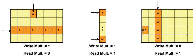
Figure 7: Various configuration of queues used by queue access fusion optimization.
