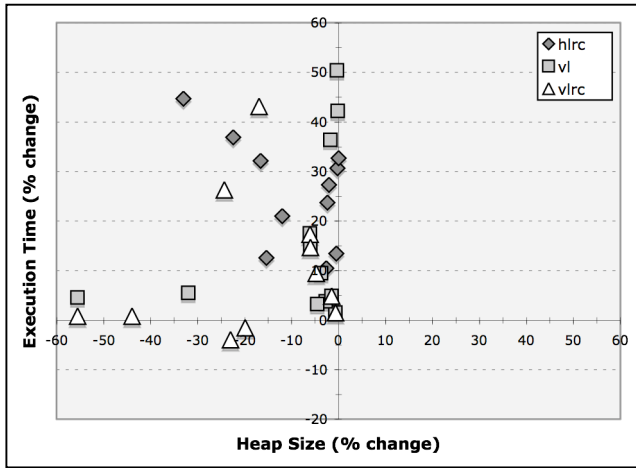
Figure 7a compares heap size change versus execution time change for the three object models, normalized against the standard horizontal object model.
