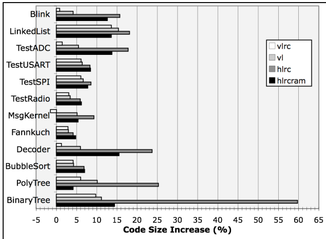
Figure 6b shows the code size increase for four object models normalized against the code size of the standard horizontal layout. (smaller is better)
