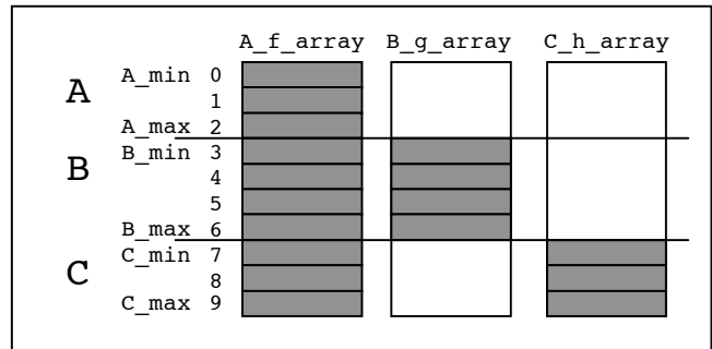
Figure 2b: Vertical object layout for the example (only classes A, B, C shown). Each field is represented by an array and only the occupied portion is stored. Preorder numbering gives objects of type A ids 0-2, B 3-6, and C 7-9.
