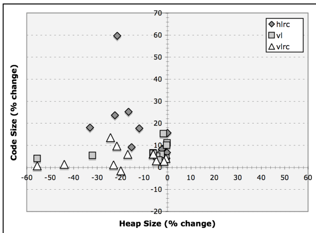
Figure 7c compares heap size change versus code size change for three object models, normalized against the standard horizontal object model.
