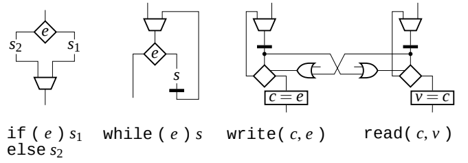
Figure 9: The translation of statements in our language.
