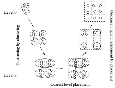
Figure 1: V-shape multi-level simulated annealing coarse placement framework
