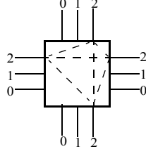
(c) Switching Block, F_s = 3
