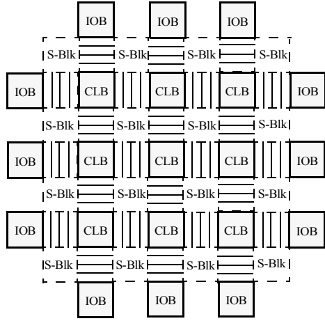
(a) Island-style FPGA Routing Model
