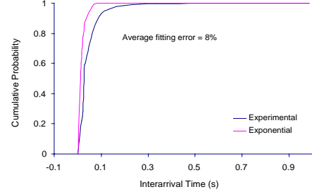
Figure 6: MPEG video arrival time distribution
