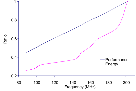
Figure 5: Performance and energy for MPEG video
