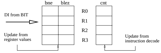
Figure 8: A four entry BDT example
