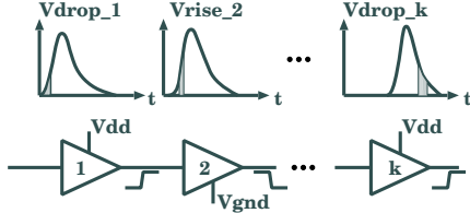
Figure 3: Illustration of a selected long critical path with worst-case supply voltage waveform
