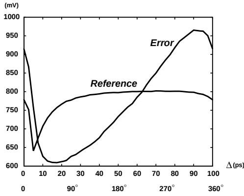
Figure 6: Determination of PD gain.
