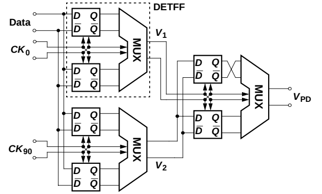
Figure 11: Phase detector.
