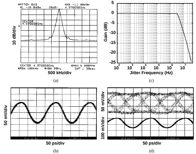
Figure 13: (a) Spectrum of the recovered clock, (b) recovered clock in the time domain, (c) measured jitter transfer characteristic, (d) recovered data and clock.
