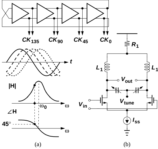
Figure 9: (a) Four-stage LC-tuned ring oscillator, (b) implementation of each stage.
