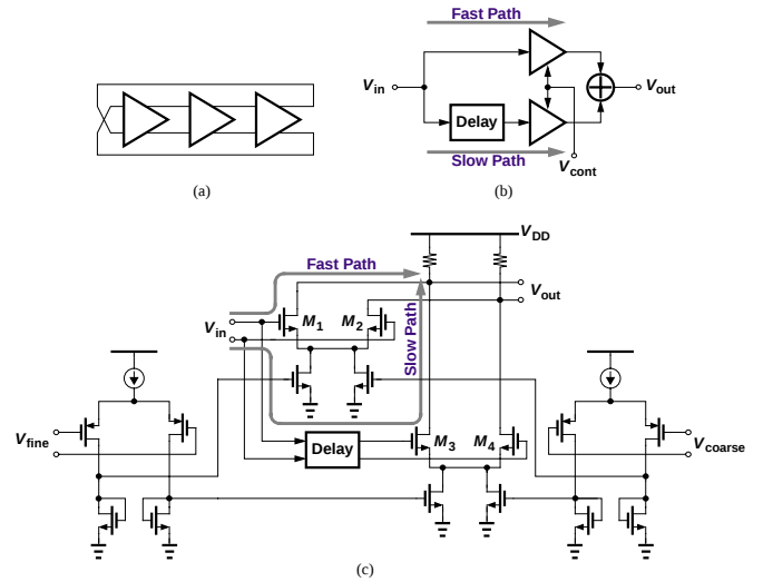
Figure 3: (a) Three-stage ring oscillator, (b) implementation of each stage, (c) transistor-level schematic.
