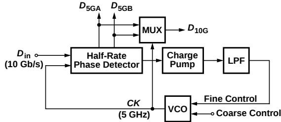
Figure 2: Half-rate CDR architecture.
