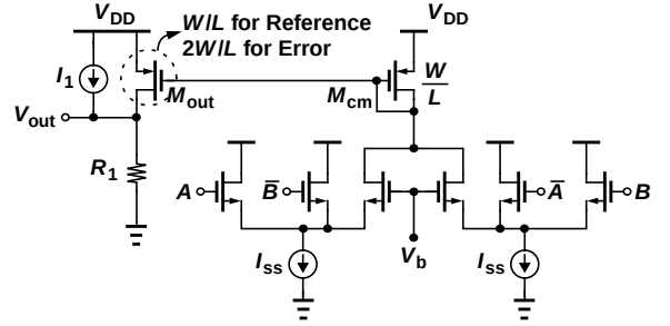
Figure 5: Symmetric XOR gate.
