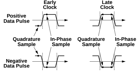
Figure 10: In-phase and quadrature samples of data pulses with early and late clock signals.
