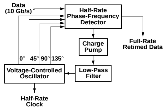
Figure 8: CDR architecture.
