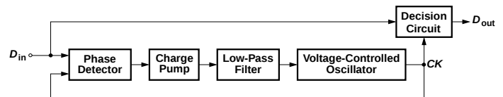
Figure 1: Generic CDR architecture.
