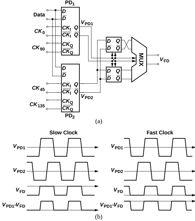
Figure 12: (a) Phase and frequency detector, (b) timing diagram in the PFD.
