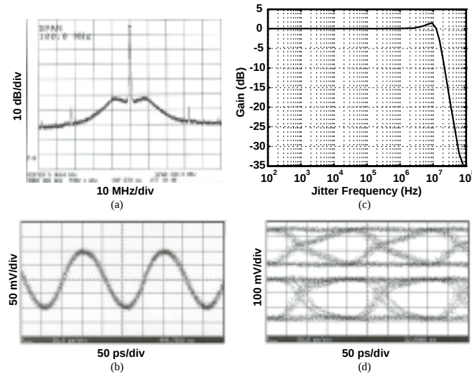
Figure 7: (a) Spectrum of the recovered clock, (b) recovered clock in the time domain, (c) measured jitter transfer characteristic, (d) recovered demultiplexed data.
