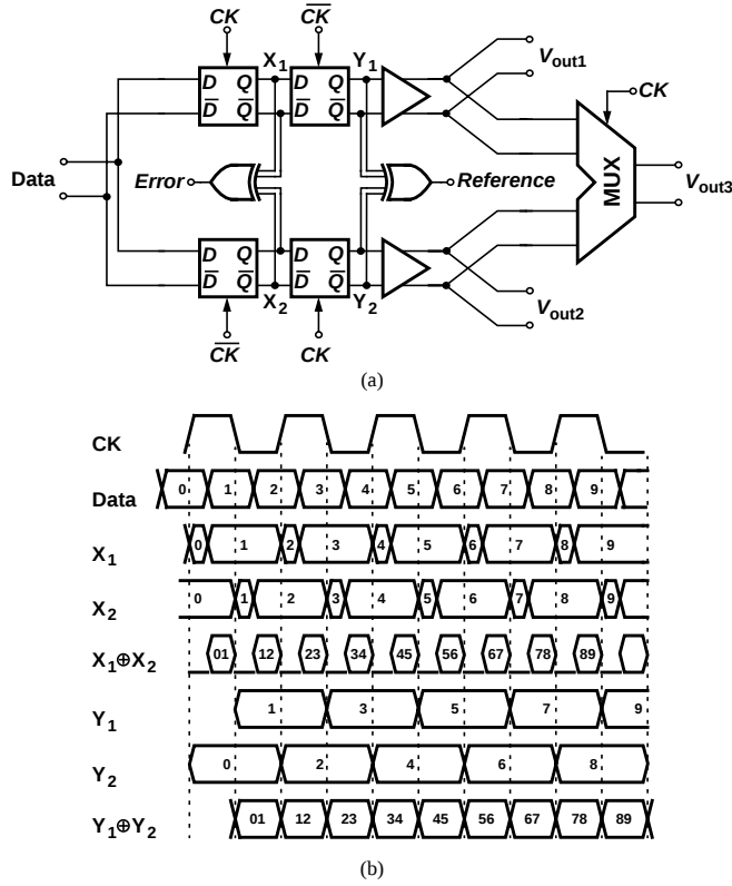
Figure 4: (a) Phase detector, (b) operation of the circuit.
