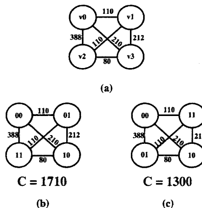
Figure 1: Example of G_A(V, E, W) Encoding.
