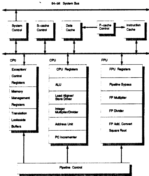
Figure 2: R4000 Processor Internal Block Diagram.
