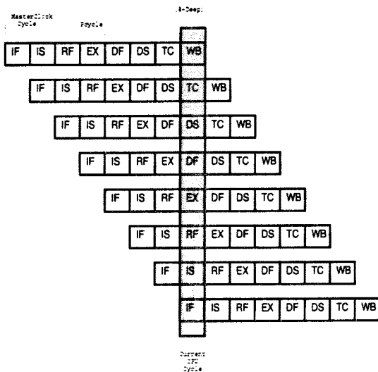
Figure 3: Instruction Pipeline Stages.
