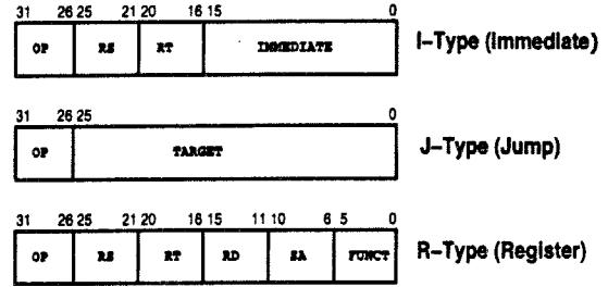
Figure 4: CPU Instruction Formats.
