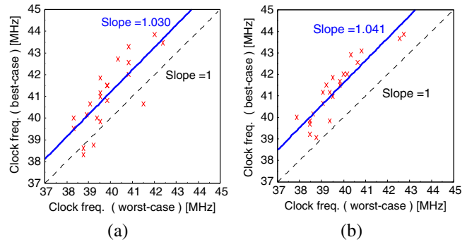
Fig. 6. (a) Variation-aware reconfiguration using WID variations on every CLB. (b) Variation-aware reconfiguration using total WID variations on CLBs in two columns.
