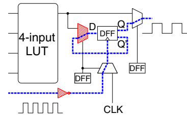
Fig. 3. Structure of a CLB. Shaded elements are used to configure a frequency divider.
