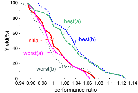
Fig. 7. Yield curves for the method (a), (b) and the initial.
