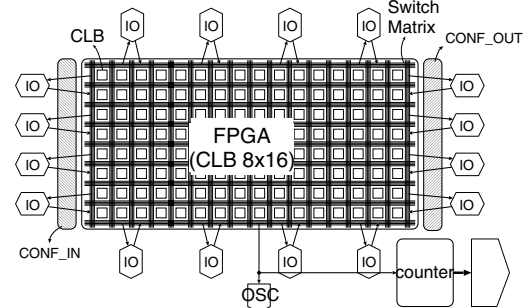
Fig. 2. Structure of the FPGA with WID-measurement capability. The counter modules counts the number of pulses from ring oscillators within a certain time.
