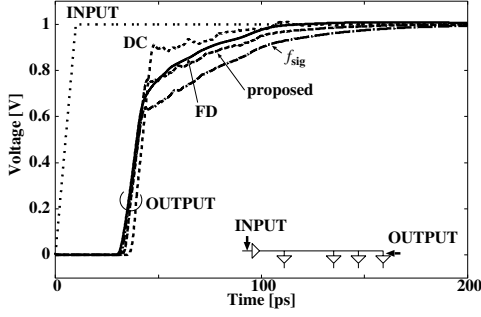
Fig. 11. Waveform at the node I of stub-bus.
