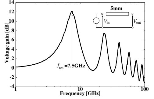
Fig. 5. transfer characteristic of a transmission-line with 5mm long.
