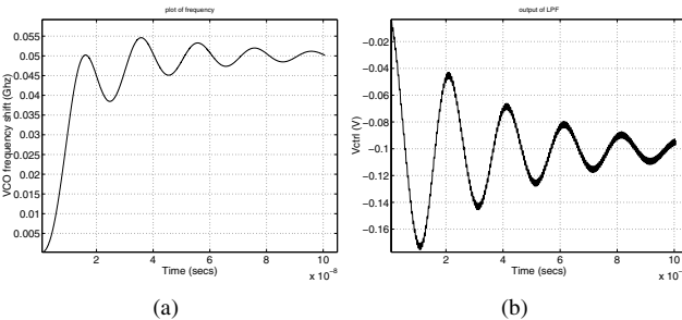
Fig. 14. Simulations with linear macromodel for new PLL
