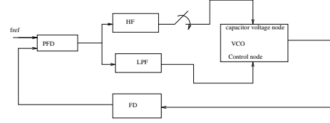
Fig. 6. New PLL Design
