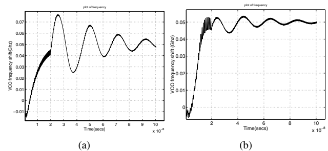
Fig. 11. Hard switching simulation for new PLL
